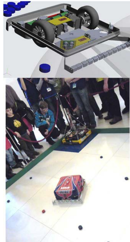
Figure 9 Puck collecting robot
