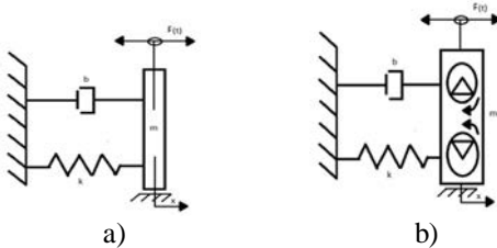
Figure 2 Mechanical system a) excitation force, b) harmonic excitation
